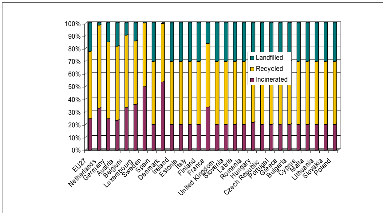
Figure 6: Shares of waste management options in scenario "50+"
