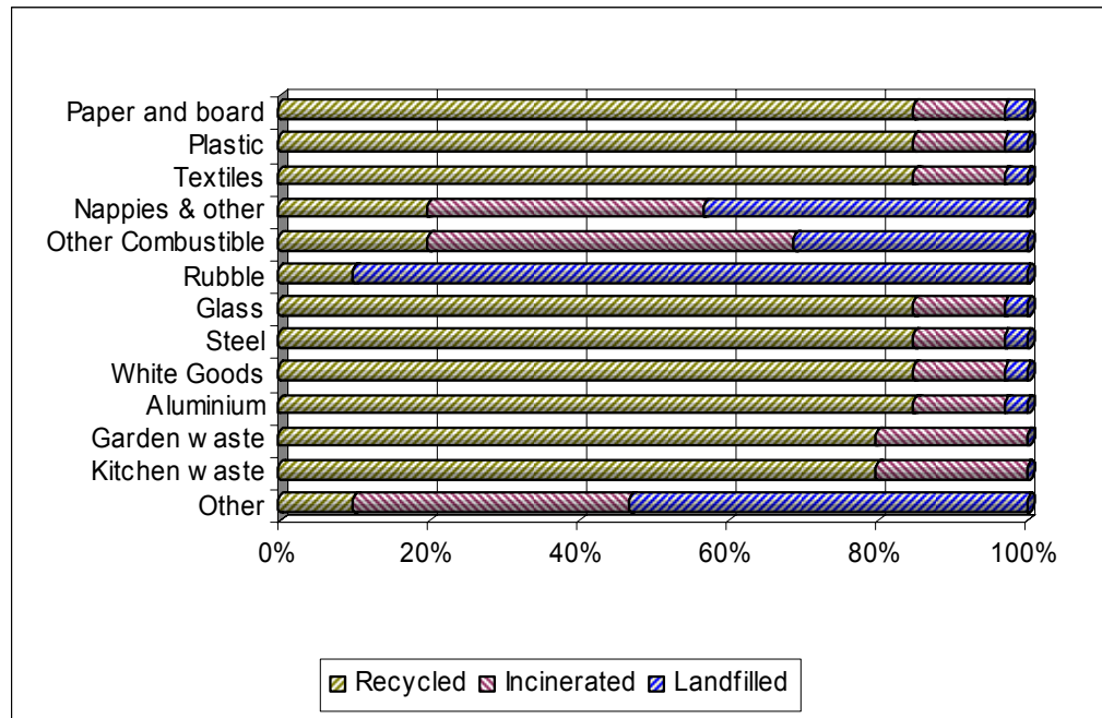
Figure 10: Recycling rates of scenario 65 in approach II
