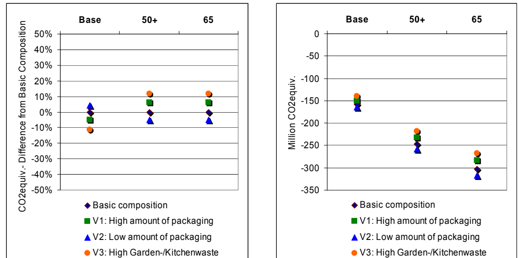
Figure 11: Development of CO 2eq saving potentials from variations of the waste composition
